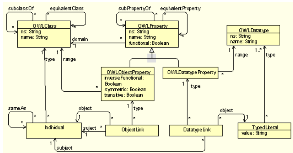
Fig. 6. OWL Lite metamodel
