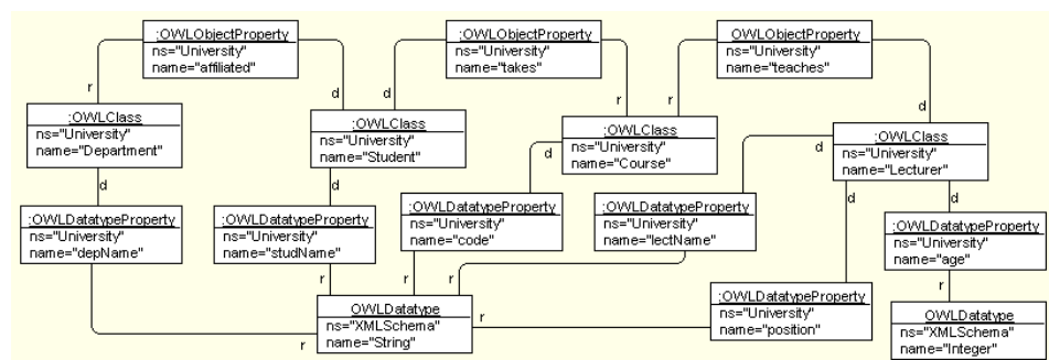
Fig. 7. University Ontology as an instance of OWL metamodel
