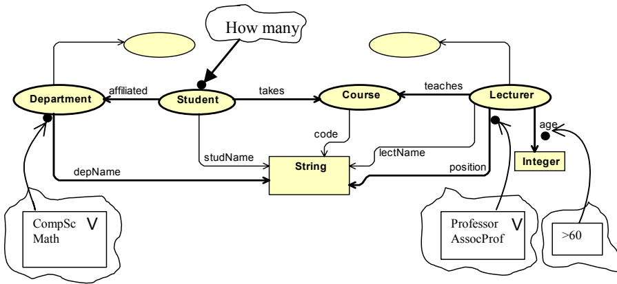
Fig. 8. Window contents of the DEMO tool showing the University Ontology
