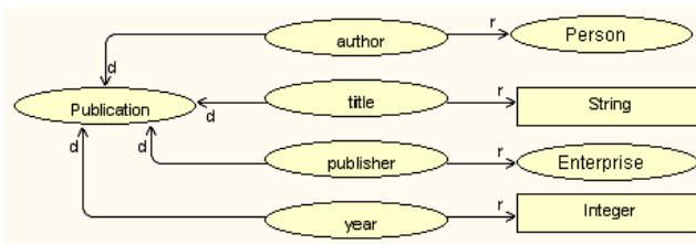
Fig. 2. Graphic representation of the “papers.owl” ontology
