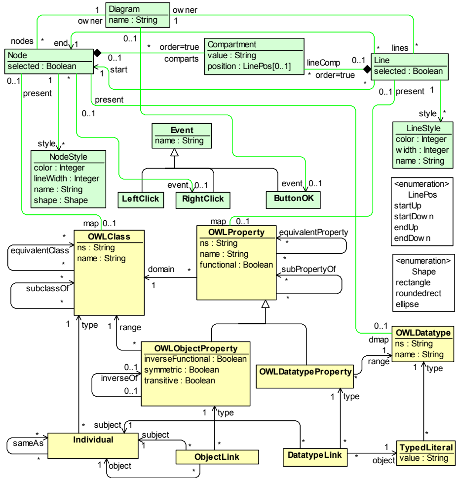
Fig. 9. The extended OWL metamodel
