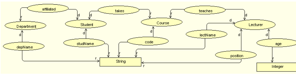
Fig. 4. University Ontology as an OWL graph (simplified)
